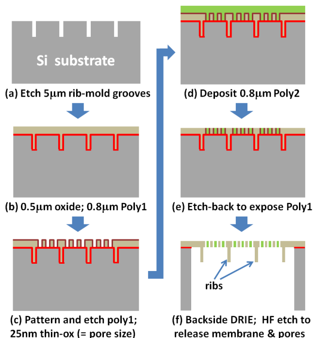
Fig. 2: Fabrication process flow for ribbed nanoporous polysilicon membranes
